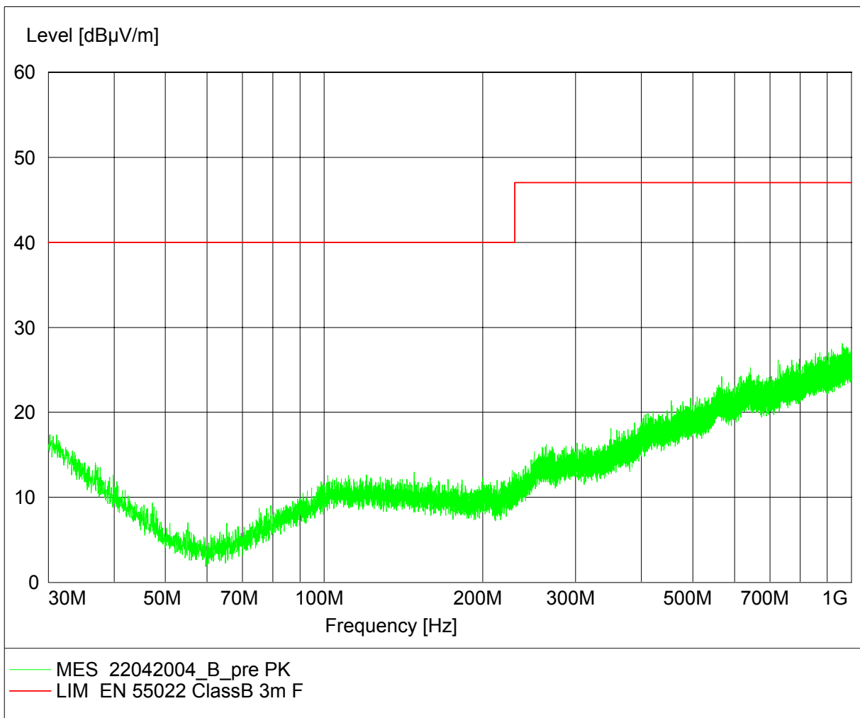
Spurious emissions 30 MHz – 1 GHz
