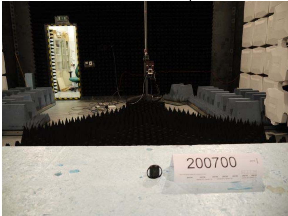
Picture 3: Transmitter Radiated emission test setup 16 GHz – 26 GHz
