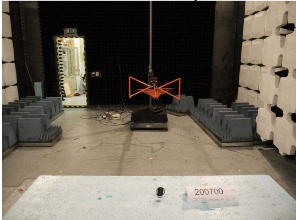
Picture 1: Transmitter Radiated emission test setup 30 MHz – 1 GHz
