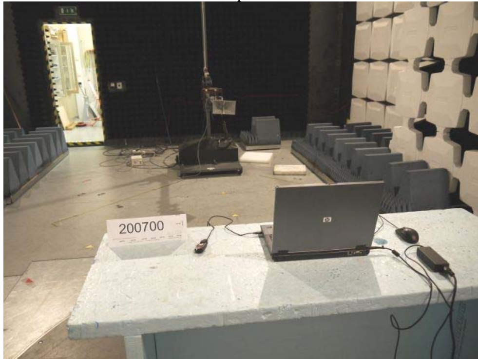
Picture 5: Radiated emission test setup 1 GHz – 16 GHz
