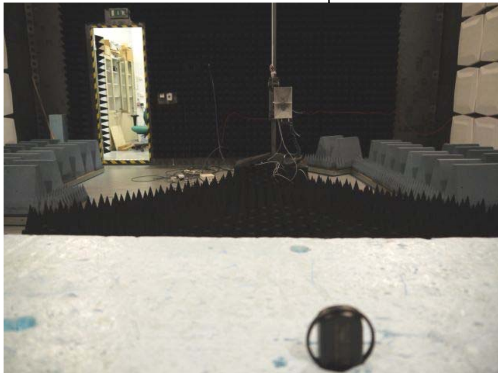
Picture 2: Transmitter Radiated emission test setup 1 GHz – 16 GHz
