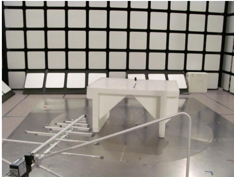
Photograph 1. Spurious emissions 30 - 1000 MHz
