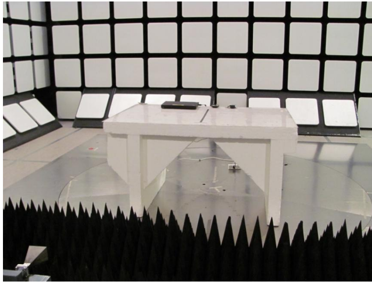
Photograph 3. Spurious emissions 18-26.5 GHz
