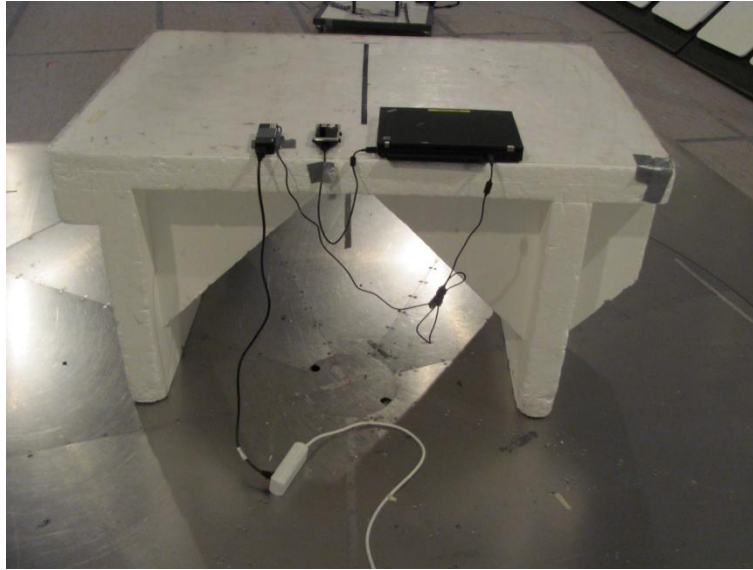
Photograph 5. EUT on table
