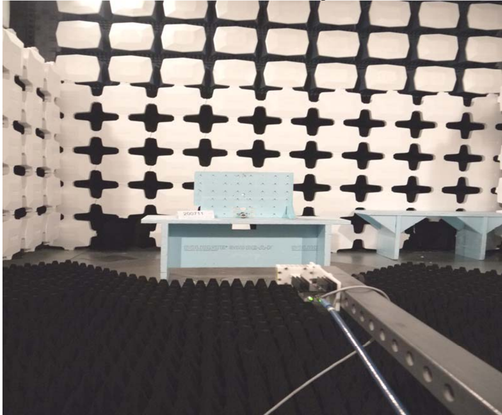
Picture 3: Transmitter Radiated emission test setup 16 GHz – 26 GHz
