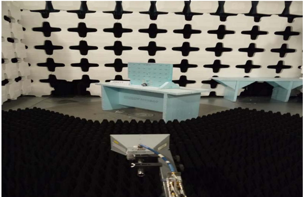
Picture 2: Transmitter Radiated emission test setup 1 GHz – 16 GHz
