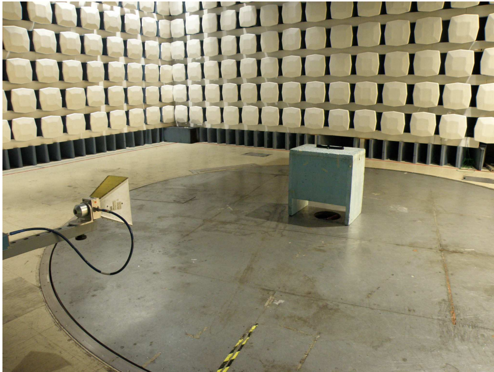
Photograph 1 Field strength of fundamental test setup
