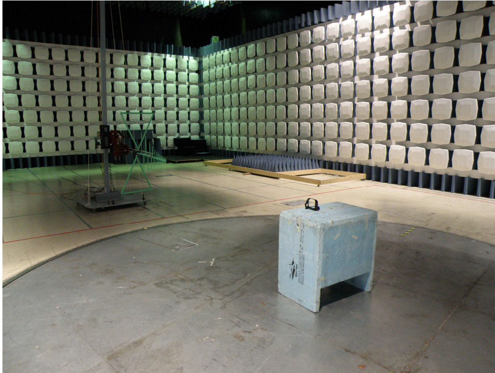
Photograph 2 Radiated spurious emissions test setup (IC 4627-1).
