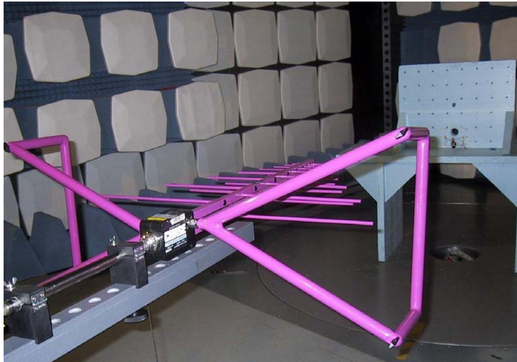
Picture 1: Spurious emission and field strength measurement setup
