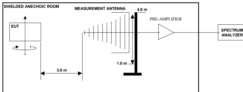
Picture 5: Test setup for radiated spurious emissions measurement 30 MHz - 1 GHz frequencies
