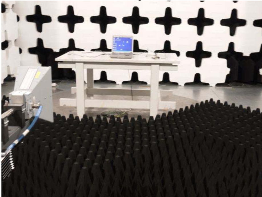
Picture 4: Radiated emission test setup 1 GHz – 16 GHz
