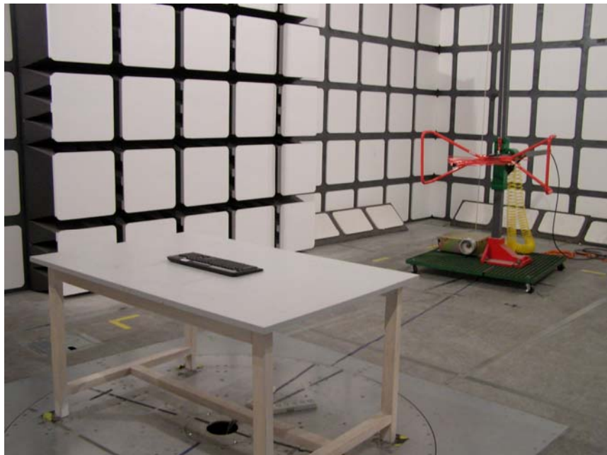
Radiated Emission (30-1000 MHz) - Rear View
