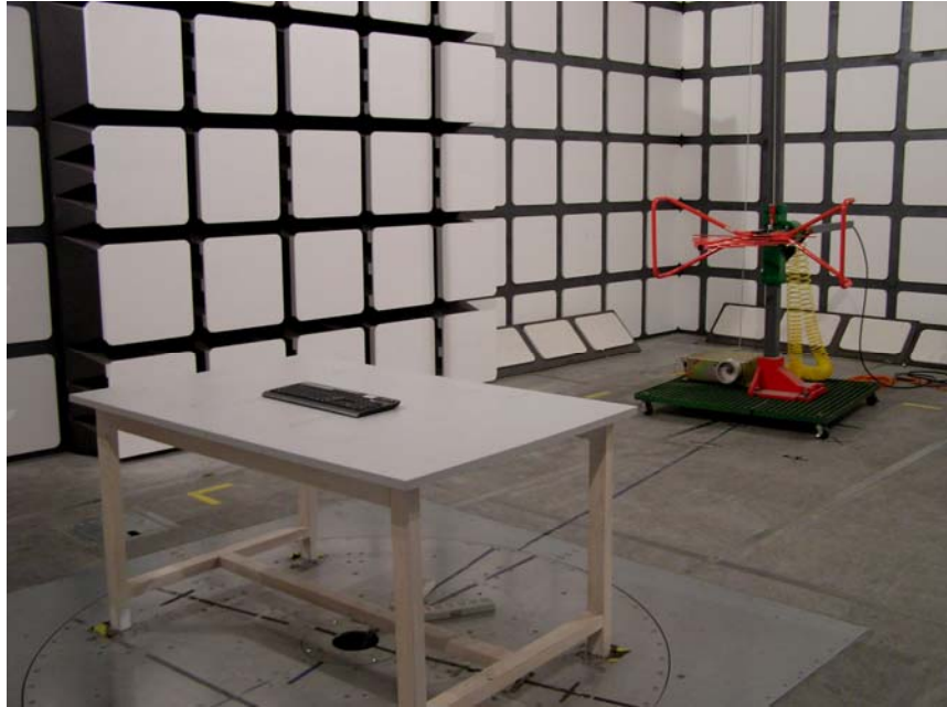
Radiated Emission (30-1000 MHz) - Front View
