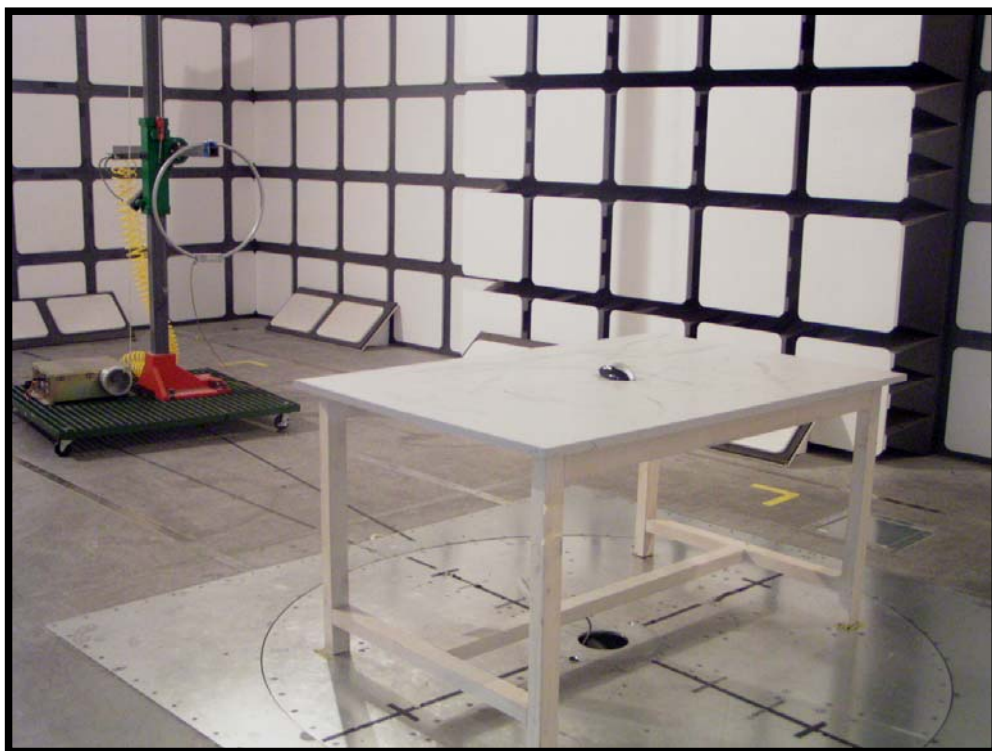
Radiated Emissions - Rear View for Fundamental
