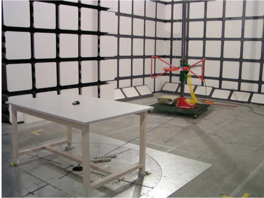
Radiated Emission-Front View (2)
