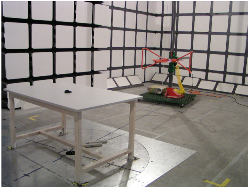
Radiated Emission-Rear View (2)
