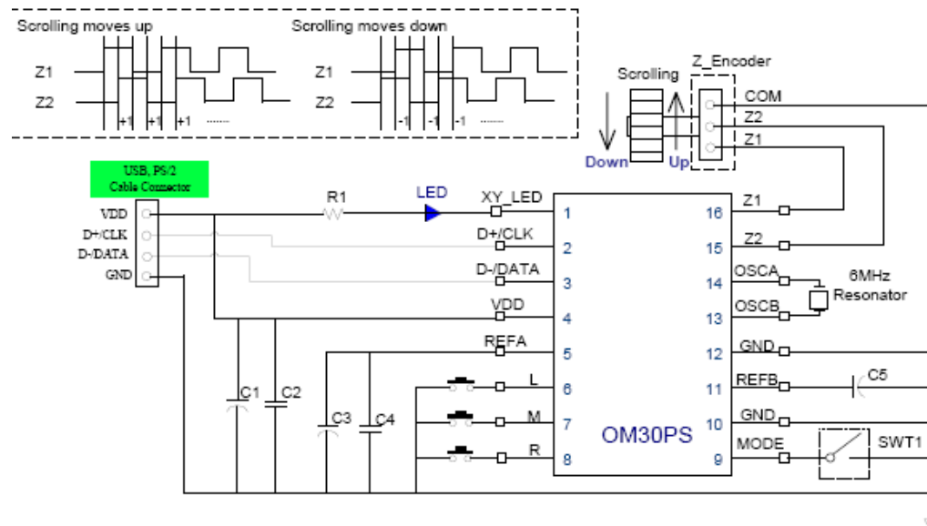
Figure 8-1 MODE-I for Basic Circuit
