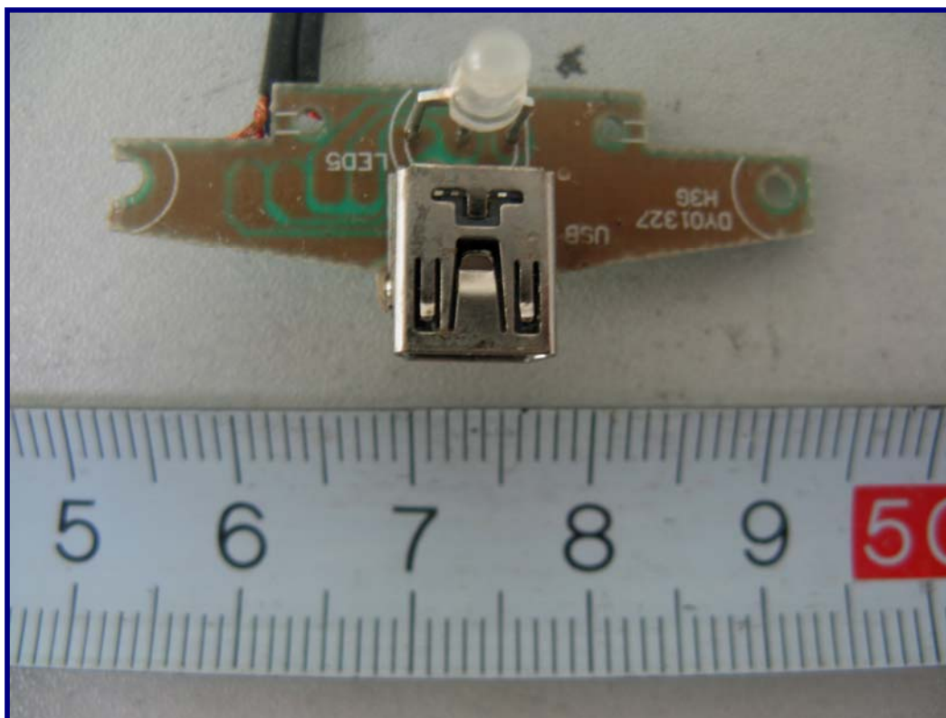
EUT- Interface Board Components View
