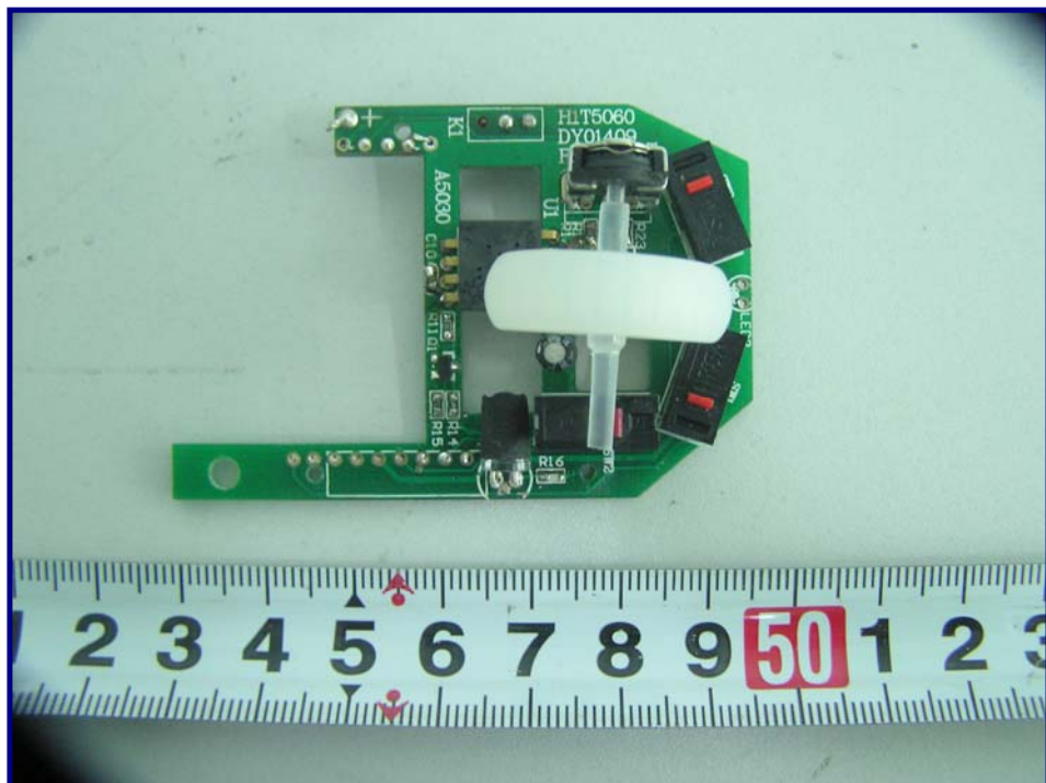
EUT - PCB 2 Components View
