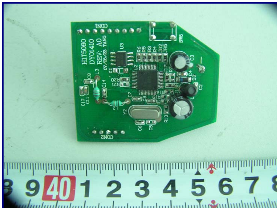
EUT - PCB 1 Component View
