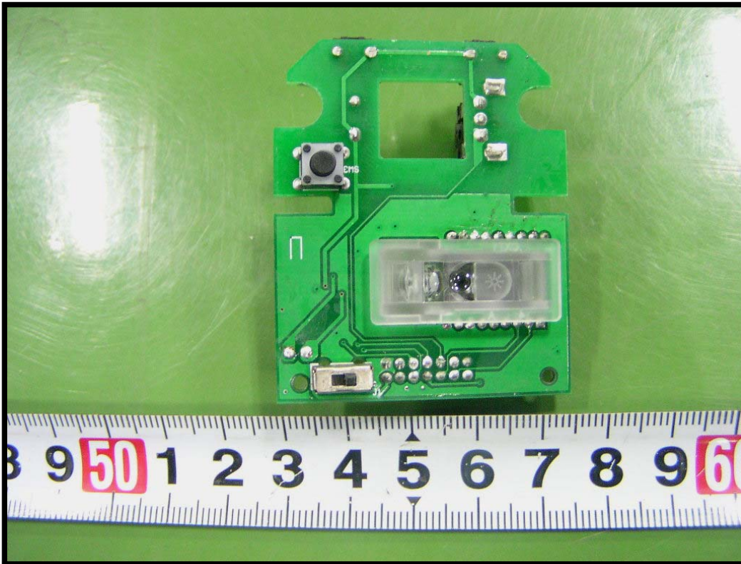
EUT - Control Board Component Bottom View
