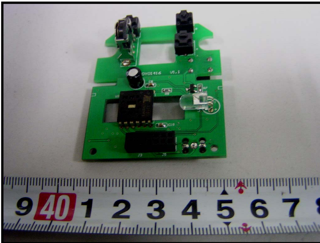
EUT- Control Board Components Top View
