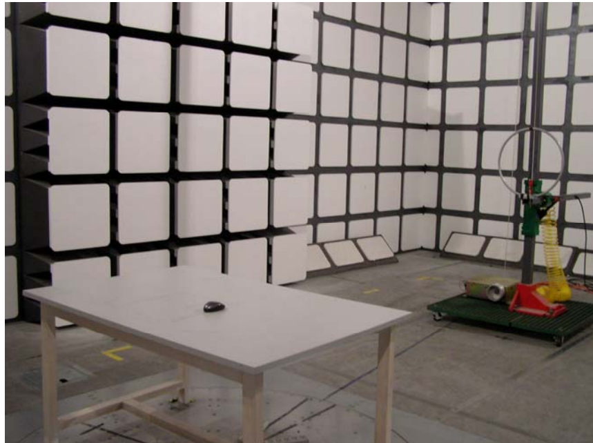
Radiated Emission (Below 30 MHz) - Front View
