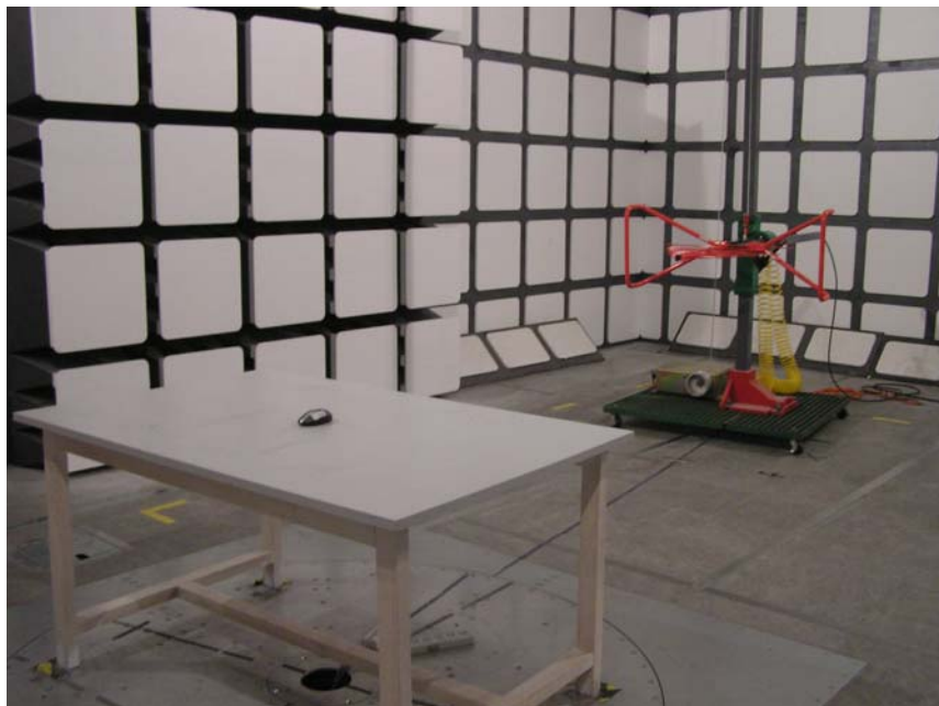
Radiated Emissions (30-1000 MHz) - Rear View
