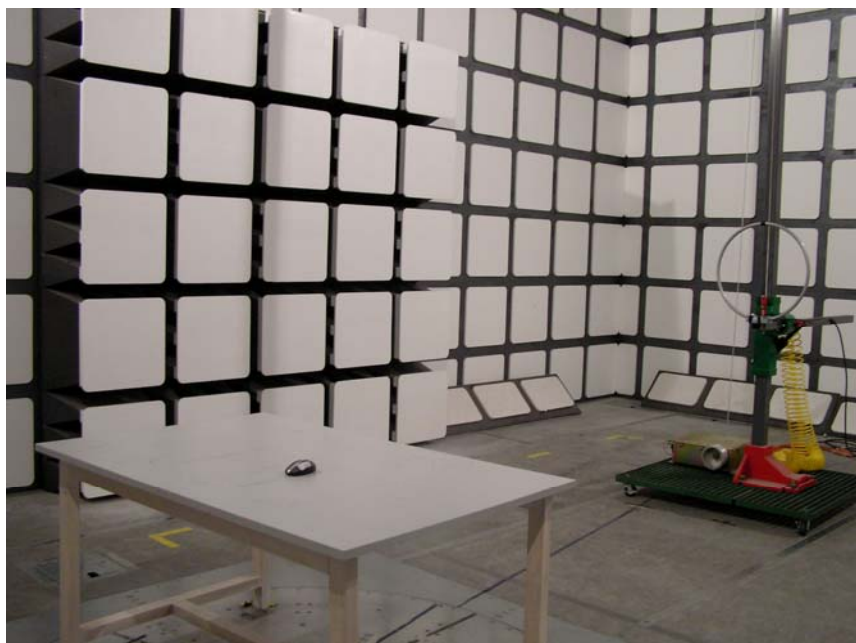
Radiated Emission (Below 30 MHz) - Rear View
