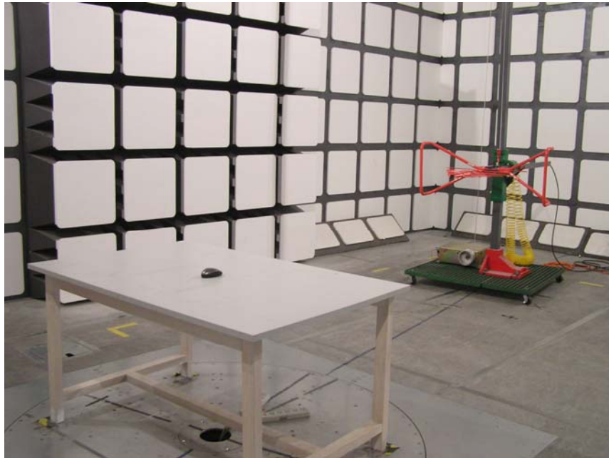
Radiated Emissions (30-1000 MHz) - Front View
