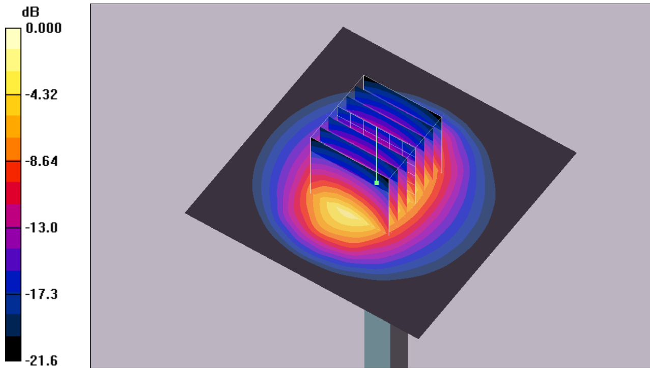
0 dB = 5.55mW/g
