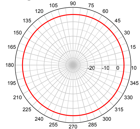
MRM3 @ 5500 MHz – Azimuth Plot
