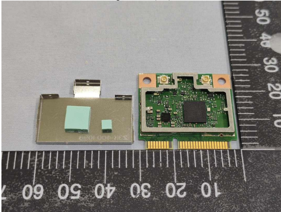
Internal Photos WPEQ-268AXI(BT) Pic 1
