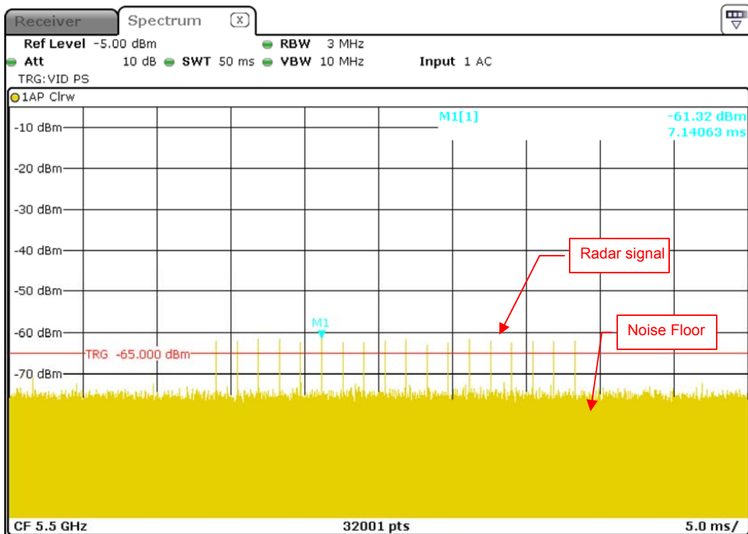
Radar Signal 0
