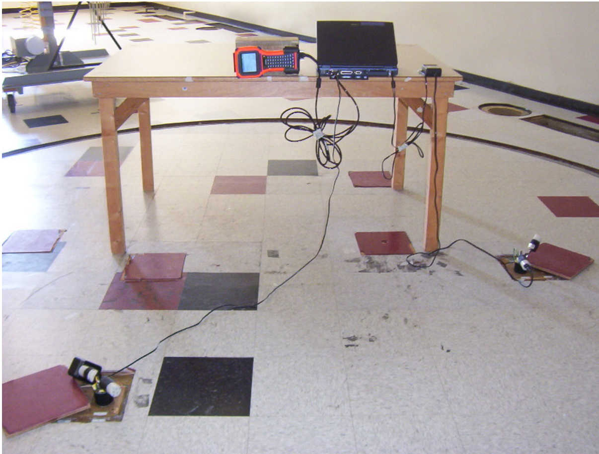
Photo 3: Radiated Emission Test Setup – Side Orientation, Front View
