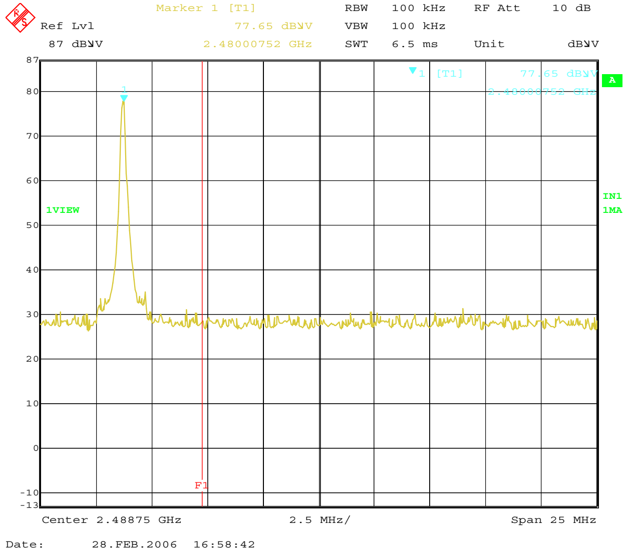
Plot 2: JETT.XL Channel 79 (Highest TX)
