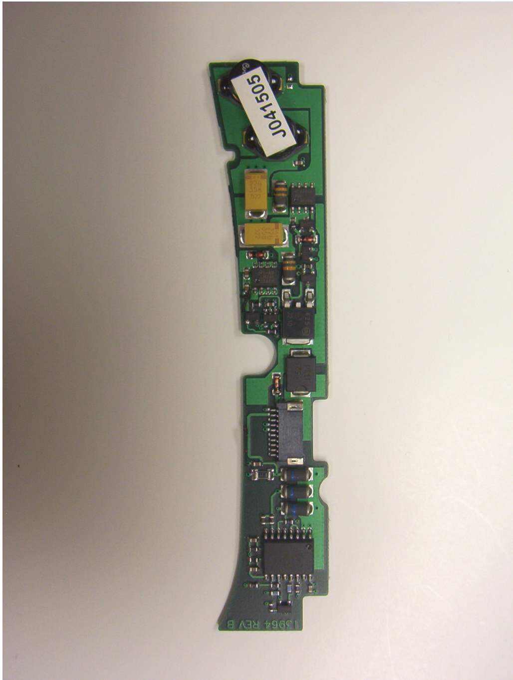
Photo 3: Charger PCB Top View
