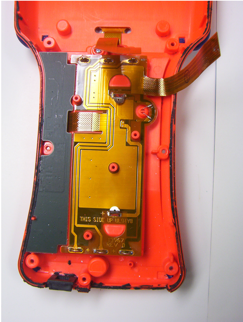
Photo 3: Power Distribution Flex Circuit View
