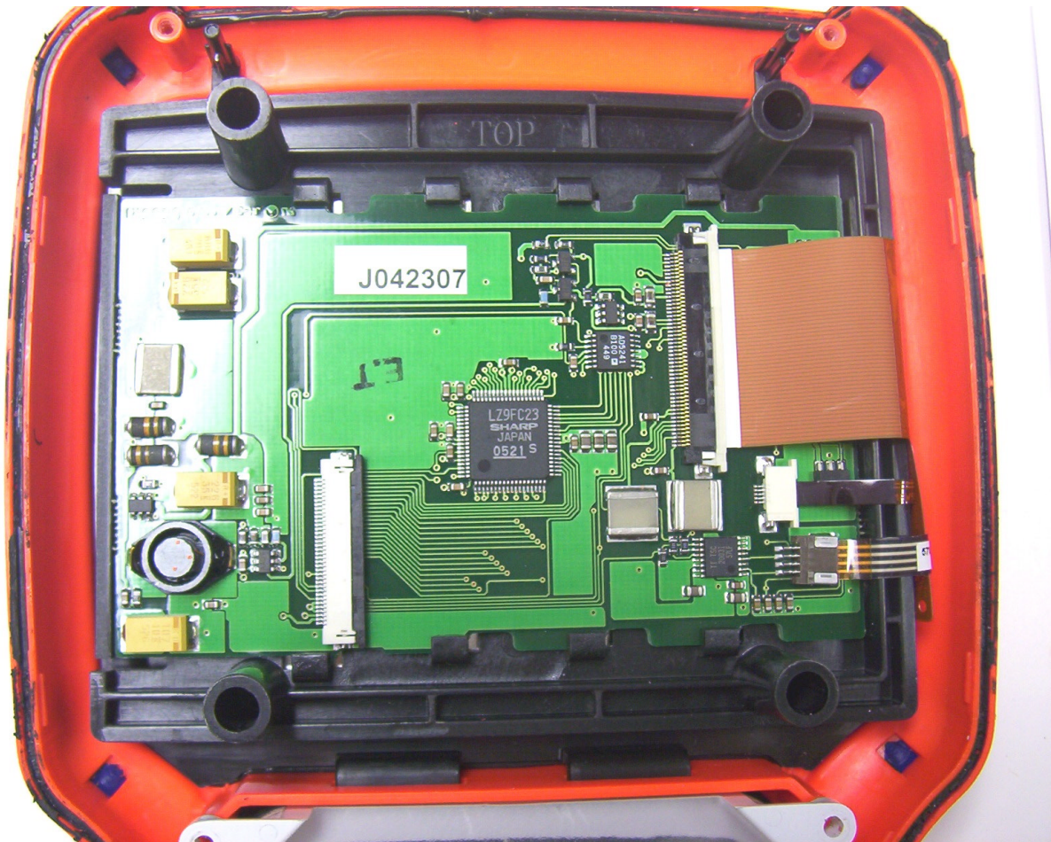
Photo 4: Sharp Display PCB View
