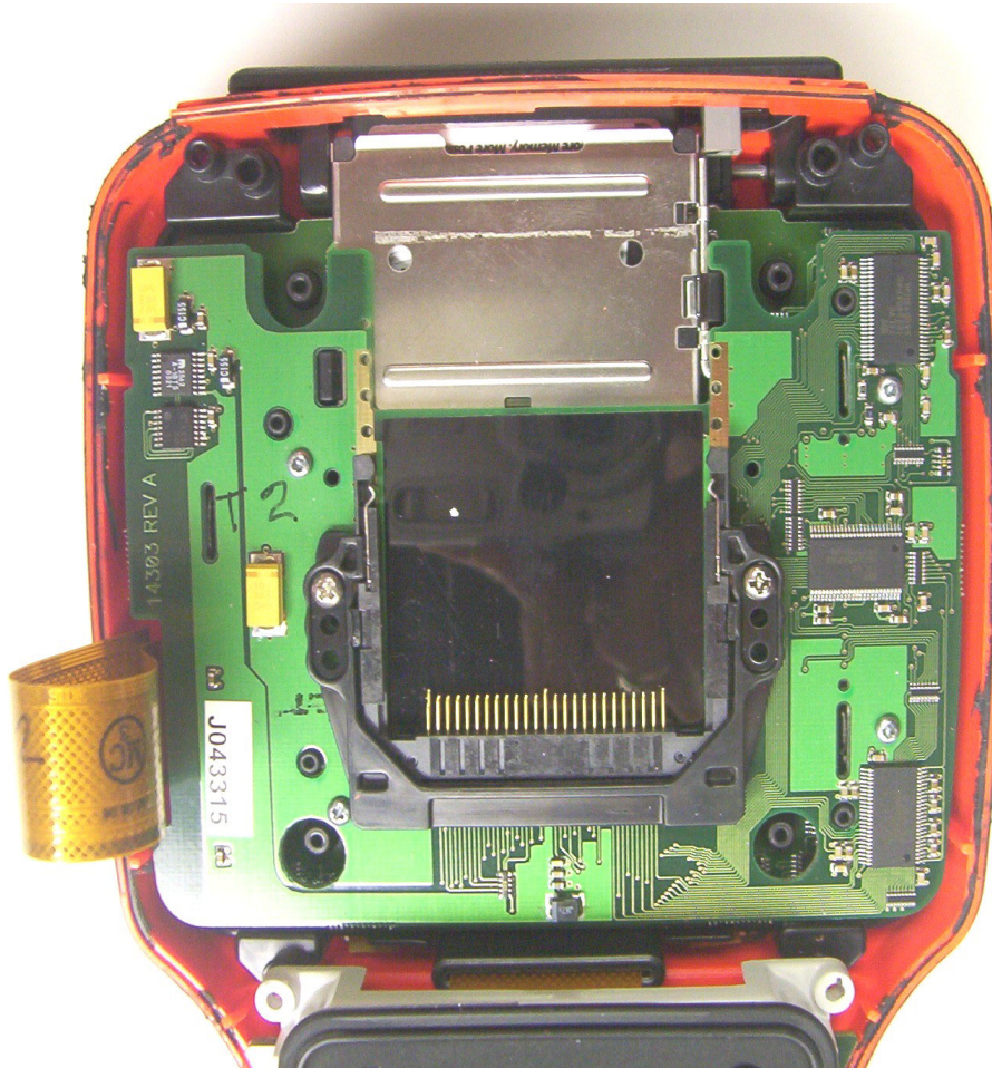
Photo 2: JETT.XL Top Half, Upper Board Bottom Close-up View
