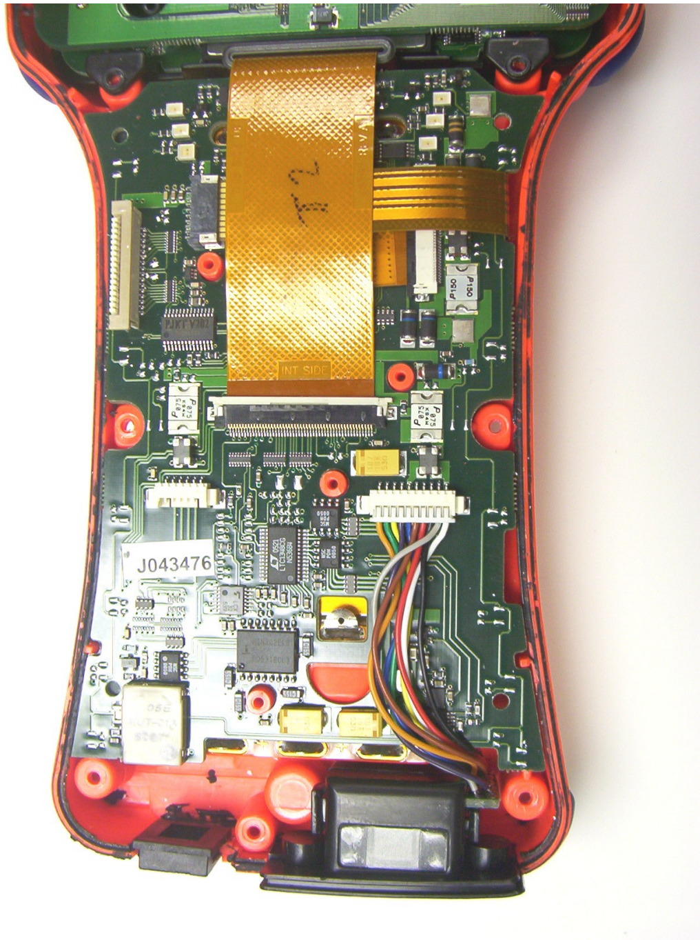
Photo 3: JETT.XL Bottom Half, Lower Top Close-up View
