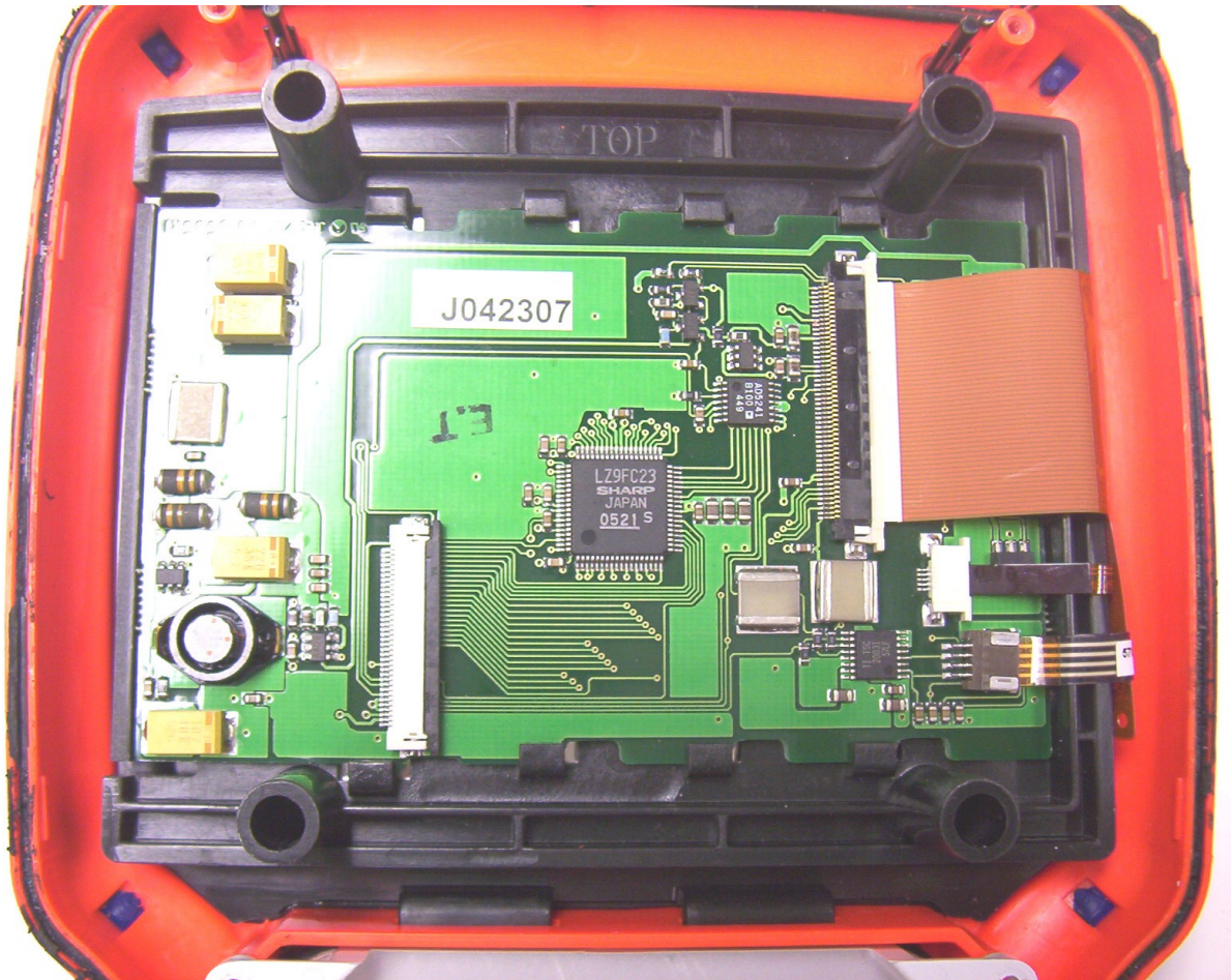
Photo 1: JETT.XL Top Half, Upper Board Top Close-up View
