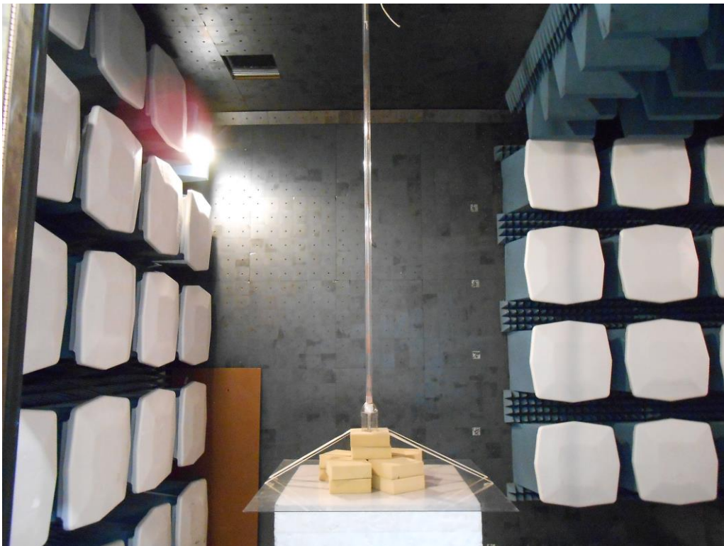
Pre-scan Transmitter
