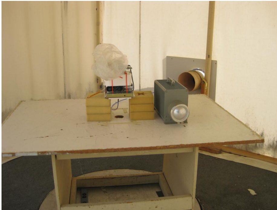
Radiated Emissions
