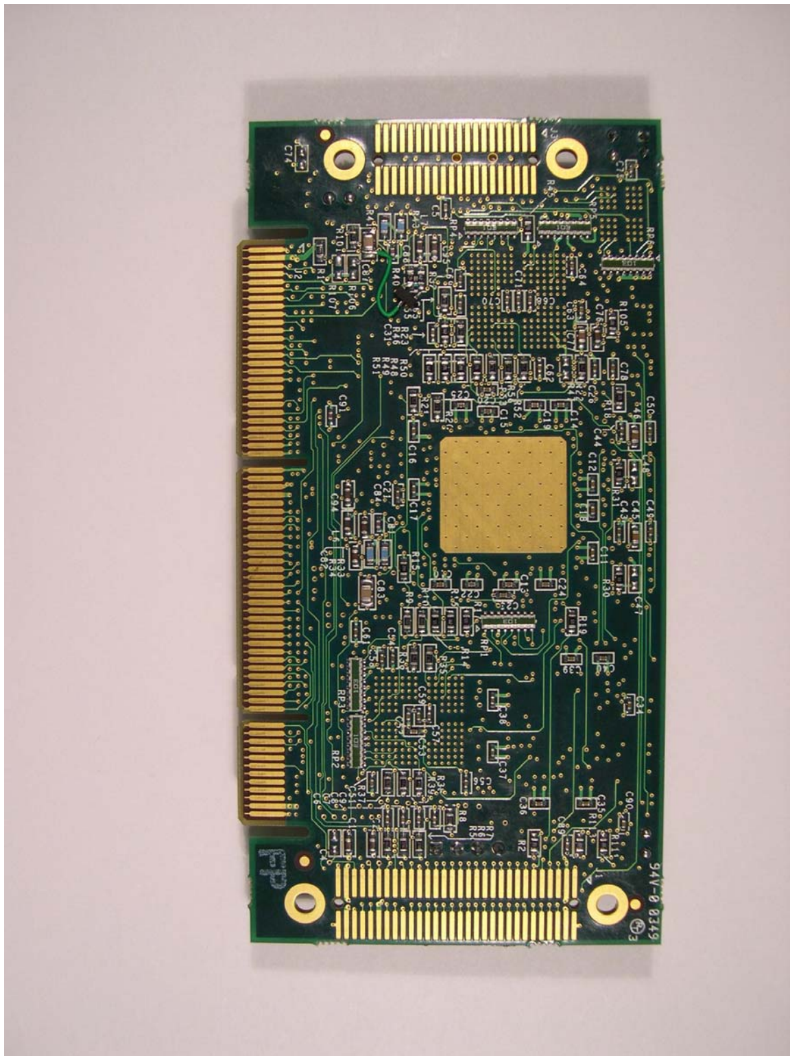
Baseband Board, Rear View
