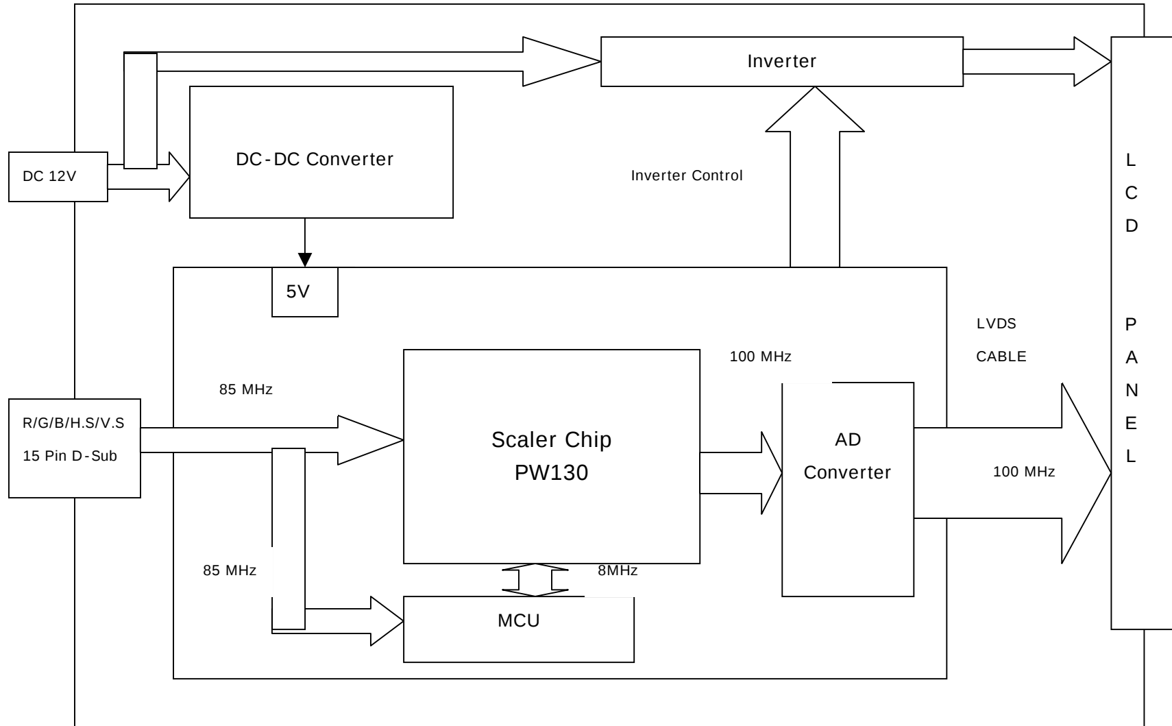
EFL -1703X Block Diagram
