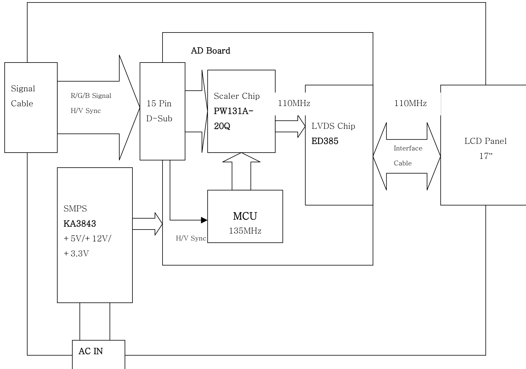
Block Diagram
