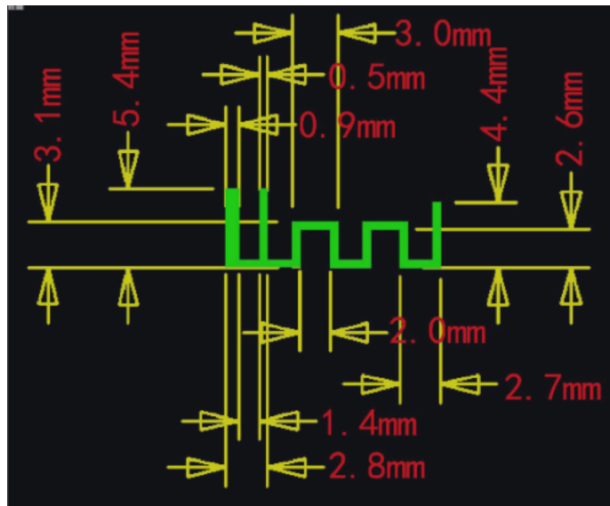
Antenna Photo & Length (mm)
