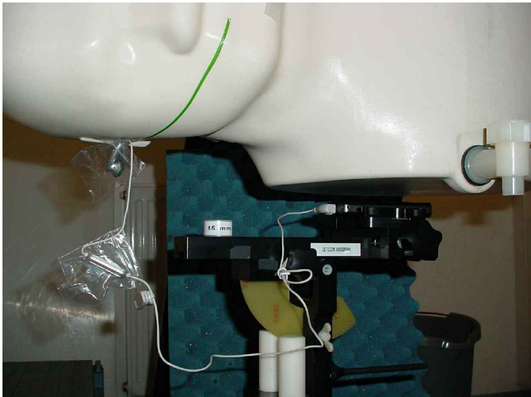
Photo 21: Test position body worn rear side (15 mm distance)
