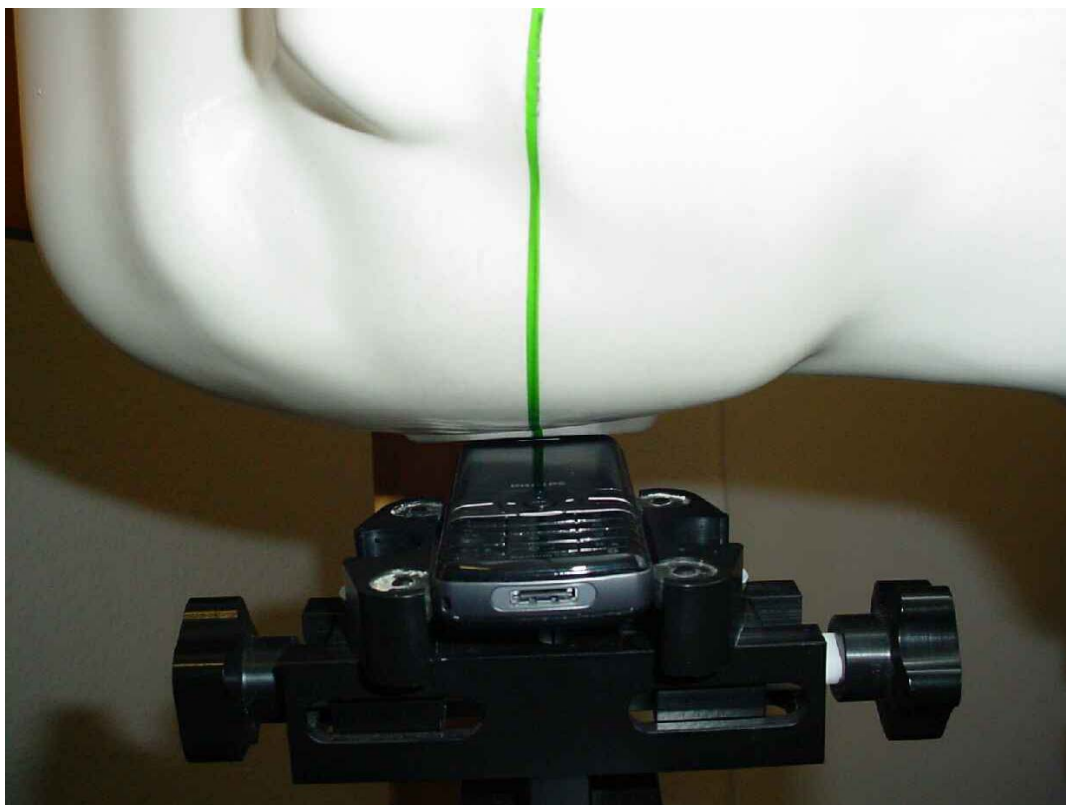
Photo 17: Test position right hand tilted 15°
