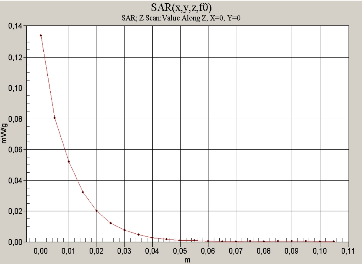
1900 MHz head
