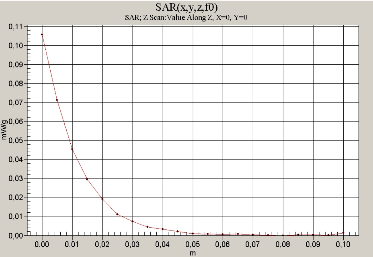
1900 MHz body
