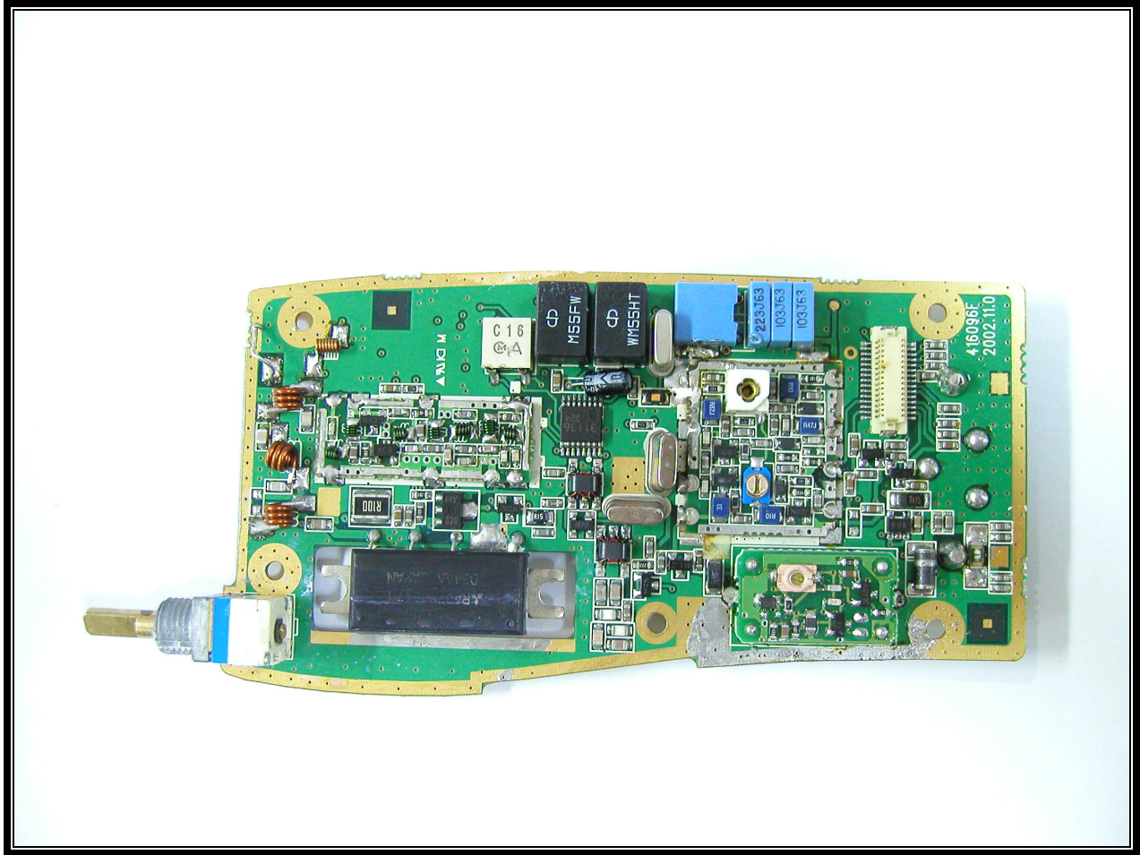
PHOTOGRAPH 16: RF UPPER 1 WITHOUT SHIELDS
