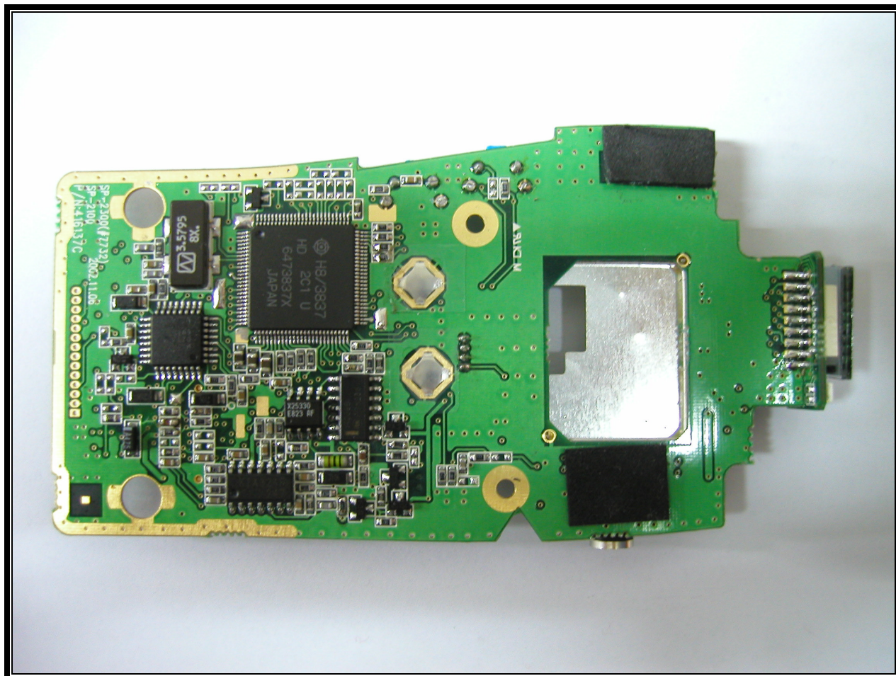
PHOTOGRAPH 13: DIGITAL PCB TOP VIEW
