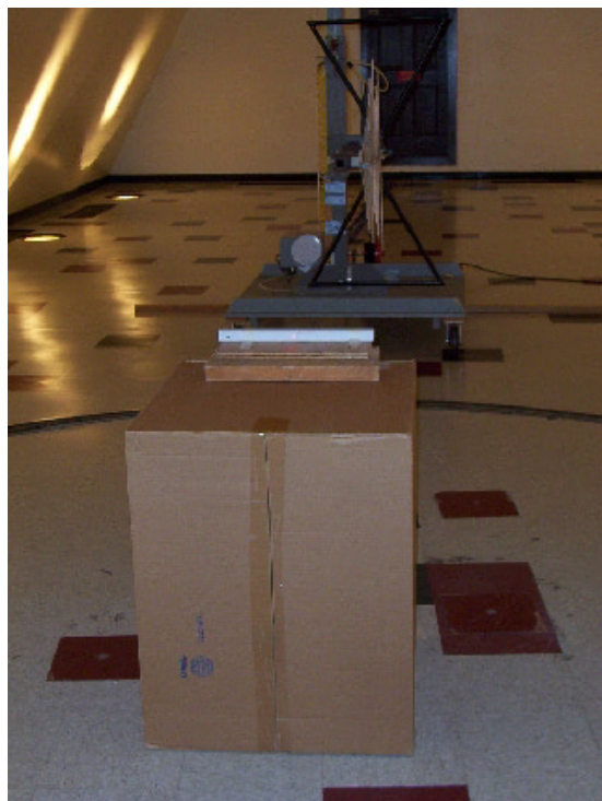
Radiated Emission Test Setup – EUT on Side, Tx Light Facing towards front
