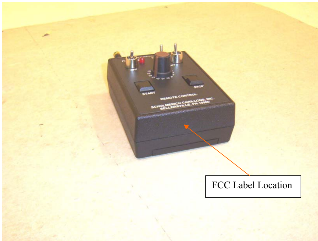
Photo 1: Generation4 Outdoor Radio Remote Control – FCC Label location
