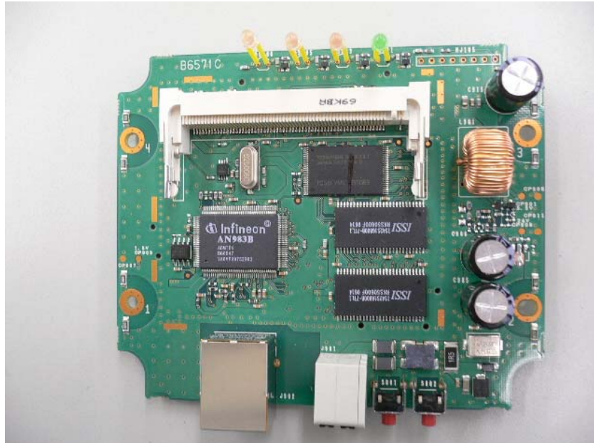
Motherboard Top (with TX removed)
