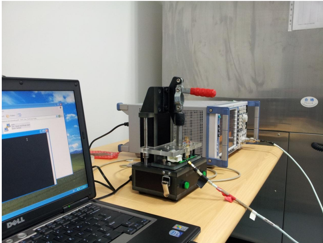
Photograph 3: Set-up for Conduct Power
