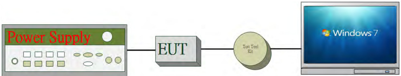
Fig. 2-1 Conducted & Radiated Emission configuration
