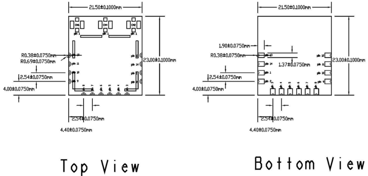
Figure 4 Mechanical Drawing
