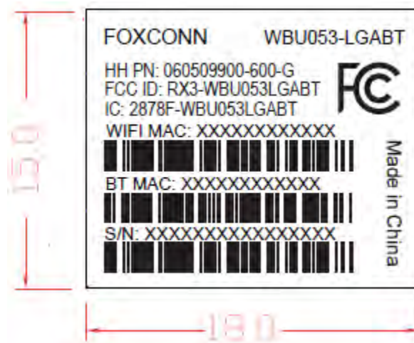
Figure 5 Label Drawing
