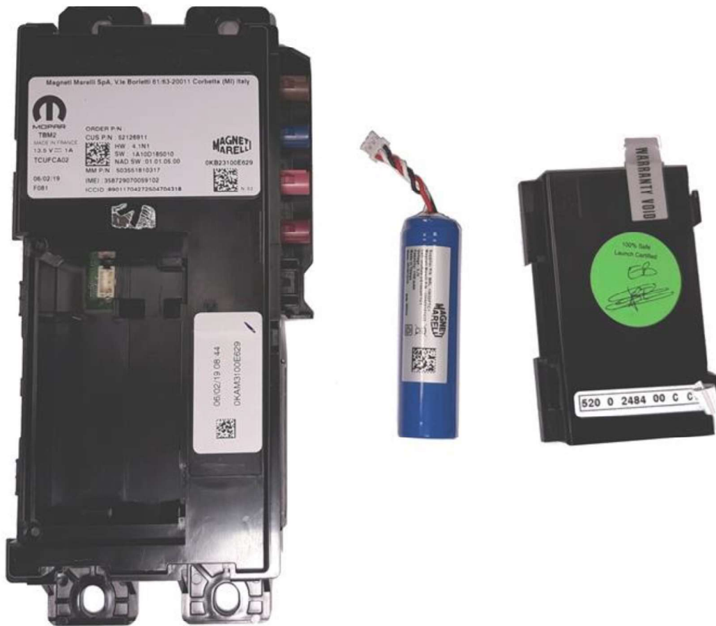
Back up battery and battery cover removed
