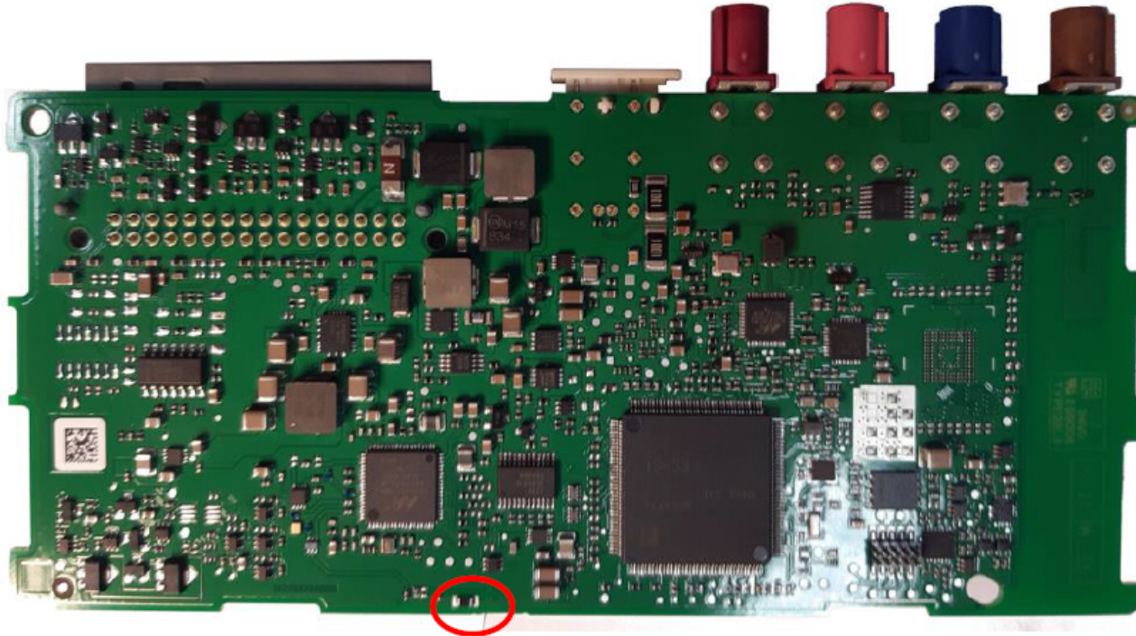
WLAN integrated antenna
