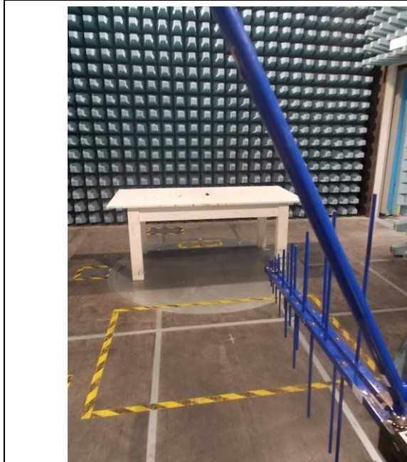
PHOTO N°2 SETUP FOR RADIATED MEASUREMENT <1GHz
