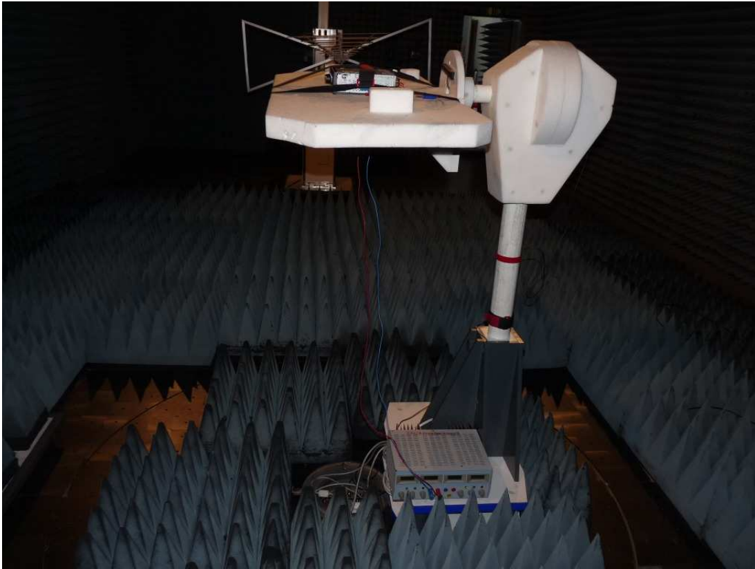
Photo 2: Test setup for radiated measurements (Enclosure, above 1 GHz)
