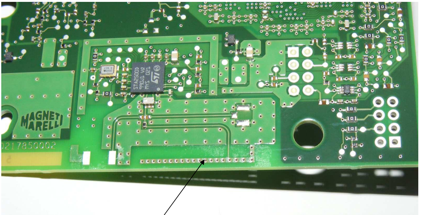
BLUTOOOTH ANTENNA
