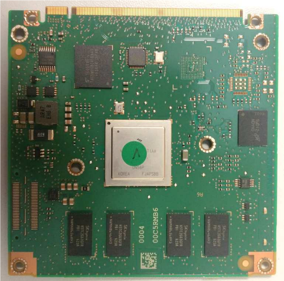
Daughterboard Top
