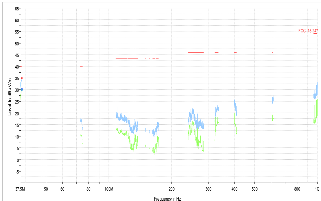
30 MHz – 1 GHz: BT GFSK (1-DH1), CH 0
